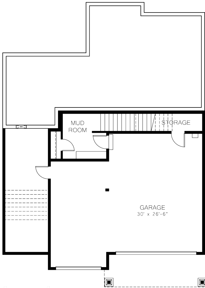
LOWER FLOOR
