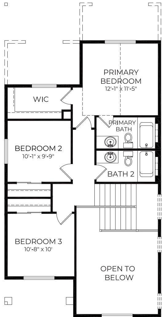
UPPER FLOOR
